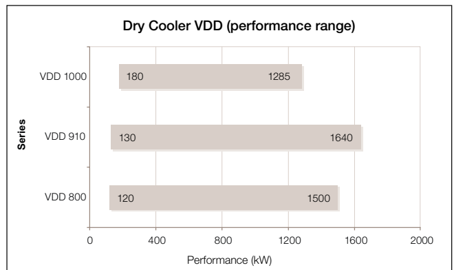
Alfa V Dry Cooler VDD series
